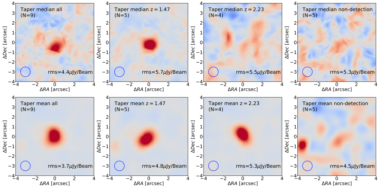
Figure C1. Postage stamps ( 8'' \times 8'' ) for the stacked continuum tapered ( \text{FWHM} = 1'' ) ALMA images. Upper and lower panels are the median and average stacks. From left to right are the stacks for different populations: all sources, only z = 1.47 , only z = 2.23 , all non-detected images (mixing galaxies at z = 1.47 at z = 2.23 ).
