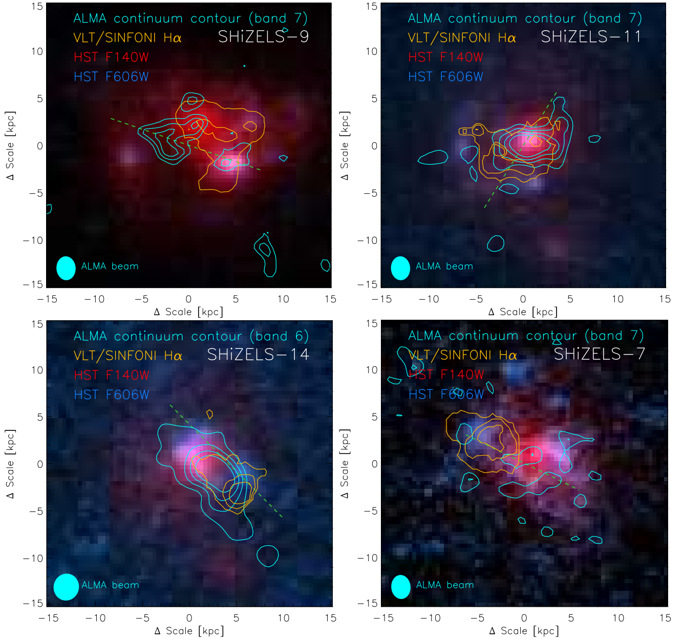
Figure 1. The HST F606W (blue) and F140W (red) true-colour composite images, including ALMA continuum contours (cyan) and H\alpha contours (orange). Contour levels are shown at 2-, 3-, 4- and 5- \sigma . The ALMA synthesised beam is shown in the lower left corner. The green dash lines show the direction of major kinematic axis ( PA_{\text{vel}} , see the velocity map in Gillman et al. 2019). The three different tracers of star formation are clearly highlighting very different regions.
