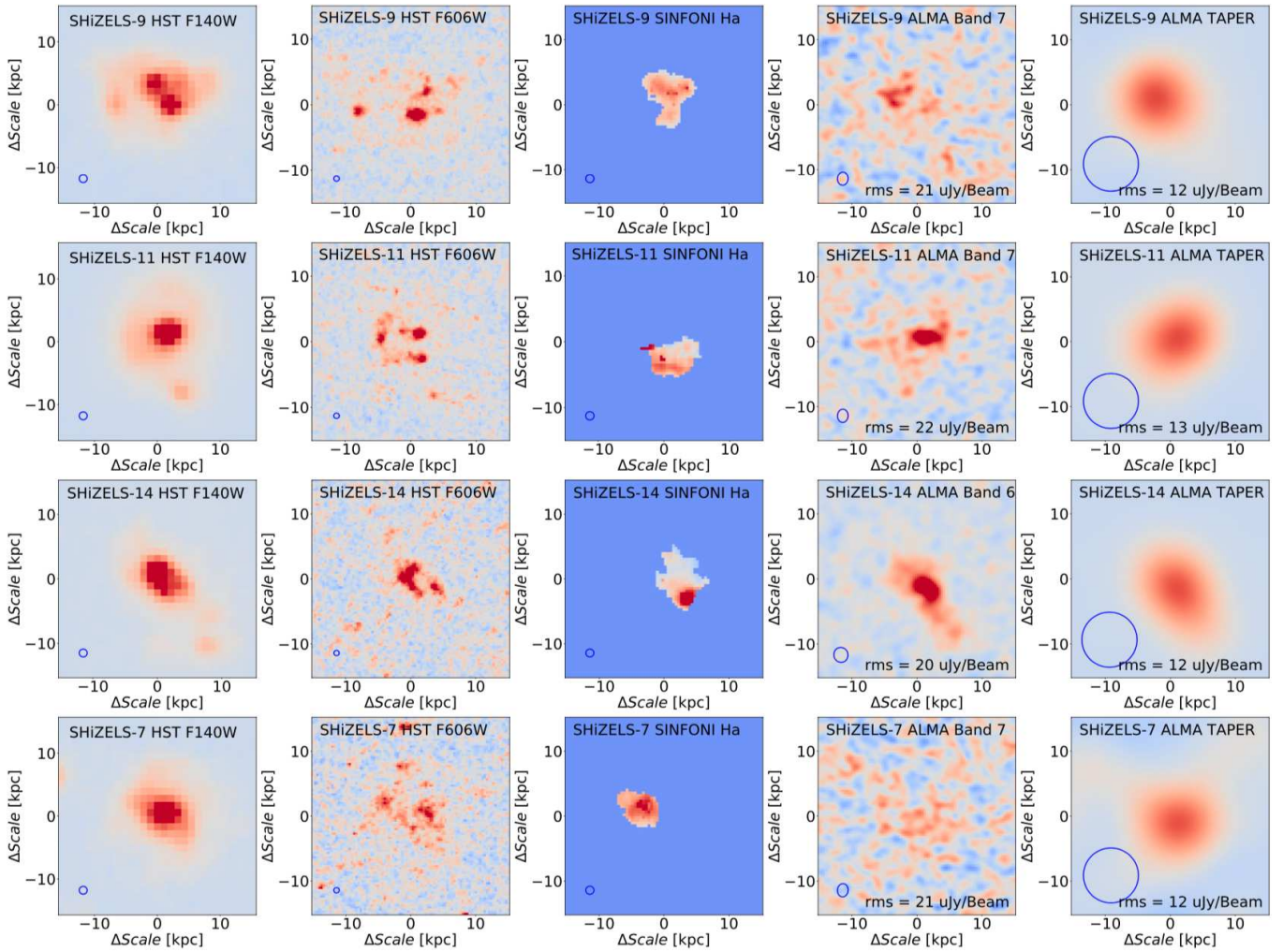
Figure A1. Postage stamp ( 30 \text{ kpc} \times 30 \text{ kpc} ) images for the SHiZELS galaxies presented in this work. From left to right images: HST F140W, HST F606W, VLT/SINFONI H\alpha moment-0, Briggs weighting ( \text{robust}=0.5 ) ALMA continuum at \sim 355 \mu\text{m} rest-frame, and tapered ALMA image (synthesised beam of \sim 1'' ) to highlight extended emission. The image shows the complexity of the different phases of the ISM in these high-redshift galaxies
