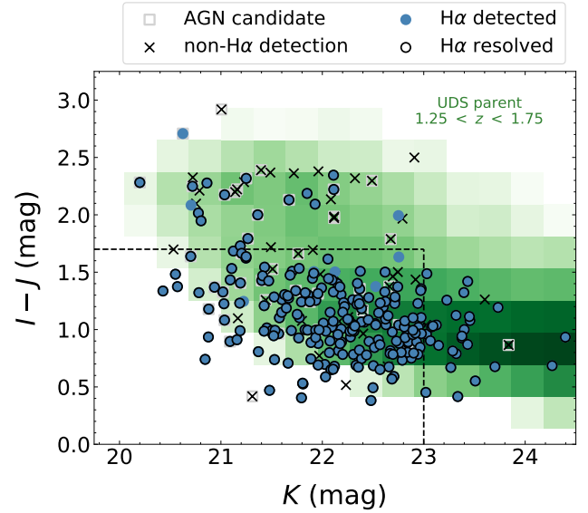
Figure 1. The KGES galaxies in the I - J versus K colour-magnitude plane. H\alpha -detected galaxies are presented as filled blue circles. A black circular outline indicates those that are also spatially resolved in H\alpha (see § 5.2). Those not detected in H\alpha are represented as black crosses. Candidate AGN hosts are indicated with hollow grey squares. The weak selection in magnitude ( K < 23 ) is indicated by the vertical dashed line. A preference was also given to targets with I - J < 1.7 (horizontal dashed line). For context, we include the distribution of a “parent” sample of \approx 24,000 galaxies from Dudzevičiūtė et al. (2020) in the UDS field (represented by a green two-dimensional histogram), with robust photometry measurements and in a similar redshift range to the KGES galaxies. The majority of H\alpha -detected and resolved KGES galaxies are bright and blue. Non-detections and candidate AGN hosts tend to be redder, but span a similar range in K band magnitudes as the H\alpha -detected galaxies.
