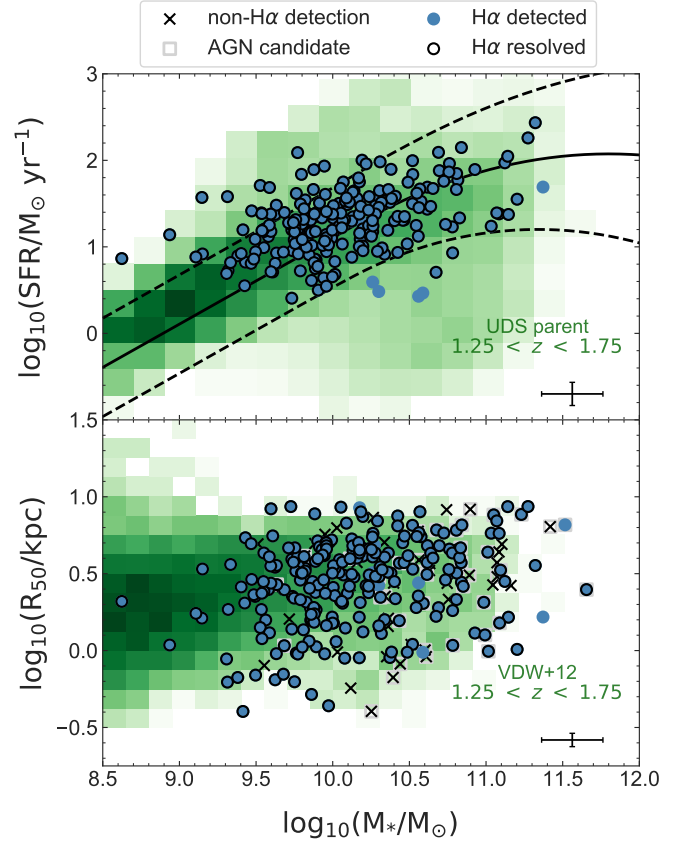
Figure 3. Top panel: The H\alpha -derived SFRs of KGES galaxies detected in H\alpha emission (excluding candidate AGN hosts) as a function of their stellar masses. Symbols are as for Figure 1. The median error bar for the KGES points is shown in the bottom right. For context, we include a two-dimensional histogram of the positions of a “parent” sample of galaxies in the UDS field. The Schreiber et al. (2015) “main sequence” of star-formation at the median redshift of the KGES galaxies and three times its corresponding 1\sigma scatter are shown as respectively solid and dashed black lines. The distribution of the KGES galaxies is consistent with typical star-forming systems at the same redshift. Bottom panel: The positions of the H\alpha -detected (and H\alpha -resolved) KGES galaxies in the stellar size-mass plane. The median error bar for the KGES points is shown in the bottom right. The spatial distribution of the KGES galaxies is in close agreement with that of a larger comparison sample of galaxies selected from CANDELS in the same redshift range ( 1.25 < z < 1.75 ) with sizes measured by van der Wel et al. (2012) from F160W ( H band) HST images, and stellar masses from the Santini et al. (2015) and Nayyeri et al. (2017) catalogues (green two dimensional histogram). The KGES galaxies have “normal” stellar sizes for their stellar masses and redshifts.
