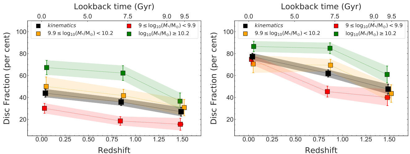
Figure 6. The fraction of discs amongst our kinematics sub-sample galaxies as a function of redshift (black squares), and also within bins of stellar mass (coloured squares). Discs as defined as galaxies with R_{\text{disc}}^2 > 0.8 and either v_{2.2C}/\sigma_{0C} > 3 (left) or v_{2.2C}/\sigma_{0C} > 1 (right). To guide the eye, we interpolate between our measurements at each redshift (dashed lines in corresponding colours) and their corresponding uncertainty (filled regions in corresponding colours). Overall, the disc fraction is a much stronger function of galaxies’ stellar masses than their redshifts.
