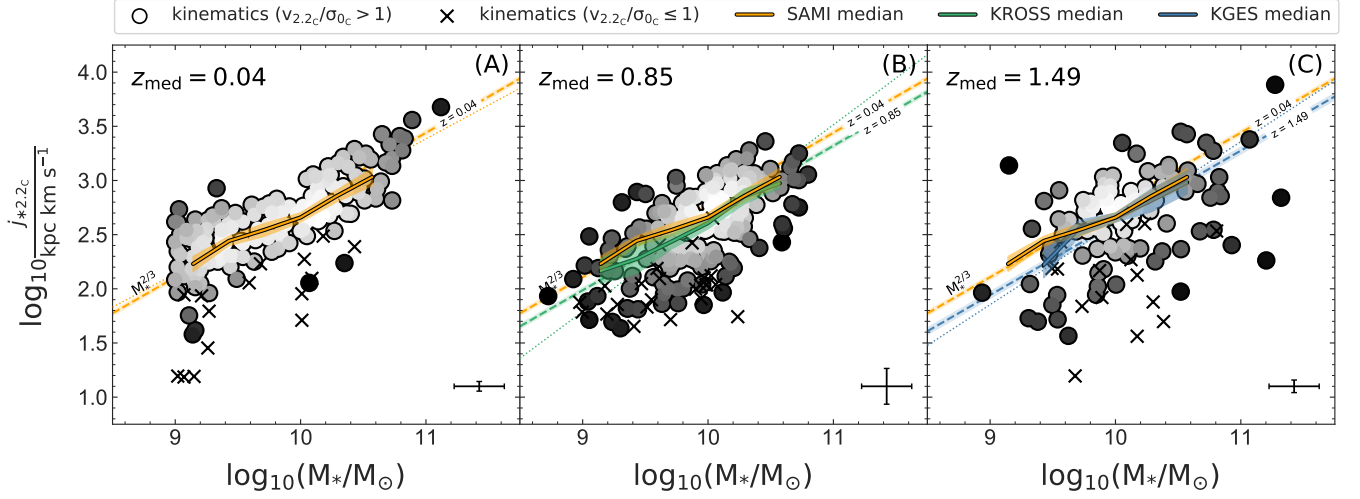
Figure 7. The specific angular momenta of star-forming galaxies in the SAMI (A, left), KROSS (B, middle) and KGES (C, right) kinematics sub-samples, as a function of their stellar masses. The galaxies span three different redshift slices at z \approx 0.04 , \approx 0.9 , and \approx 1.5 . Scatter points are colour-coded by the local spatial density of the points themselves (dark to light, low to high density; quantified via a Gaussian kernel density estimate and LOESS-smoothed). The best linear fit (with slope fixed to 2/3 ) and its 1\sigma uncertainty envelope is shown for the SAMI galaxies as an orange dashed line and filled region respectively in each panel. The corresponding best fits to the KROSS and KGES galaxies are shown as respectively a green and a blue dashed line and filled region in the middle and right panels. Similarly the median trends, and their 1\sigma uncertainty envelopes, for each sample are shown by solid lines and filled regions in the same colours. There is a small offset between the normalisation of the z = 0.04 best fit linear trend, and that for the higher redshifts galaxies. However, the median trends do not significantly differ as a function of redshift. Thus, on median average, at fixed stellar mass a massive, star-forming galaxy has the same specific angular momentum regardless of whether it resides at z \approx 0 , \approx 0.9 , or \approx 1.5 .
