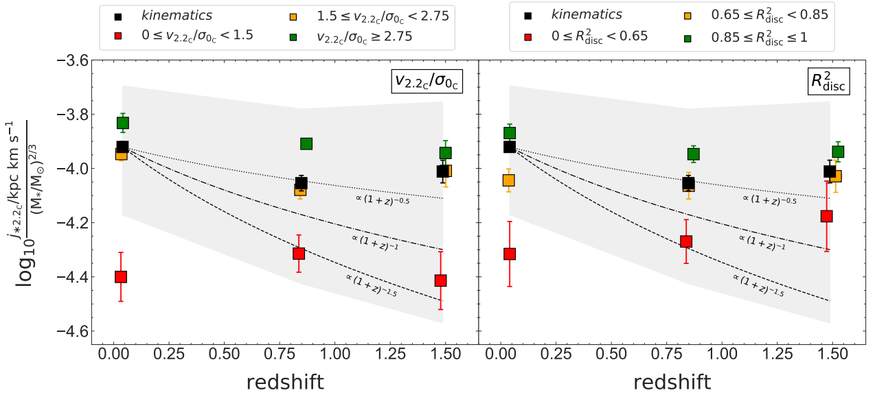
Figure 8. The median normalisation (assuming j_{*2.2c} \propto M_*^{2/3} ) of kinematics sub-sample galaxies in the specific angular momentum-stellar mass plane, as a function of their redshifts and “disciness”. The latter is quantified in the left panel by the galaxies’ (gas) rotation velocity-to-velocity dispersion ratios ( v_{2.2c}/\sigma_{0c} ), and in the right panel by how well their H\alpha velocity field is described by a two-dimensional exponential disc model ( R_{\text{disc}}^2 ; the fraction of the variation in the velocity field that is explained by the best fit two dimensional disc model). The total median normalisation at each redshift is shown by the black squares. The median normalisations at each redshift in bins of disciness are shown by the coloured squares. The bin boundaries are given in the legend of each panel. The 1\sigma scatter envelope (spanning from the 16 th to the 84 th percentile) for the normalisations at each redshift is shown as an underlying filled grey region. We linearly interpolate this between redshifts to better highlight any changes in the scatter. We also overlay tracks of j_{*2.2c}/M_*^{2/3} \propto (1+z)^{-n} , with n = 0.5, 1 , and 1.5 . The normalisation of the specific angular momentum-stellar mass relation does not evolve significantly with redshift. It is instead a strong function of a galaxy’s disciness, which is uniform across all three redshift bins.
