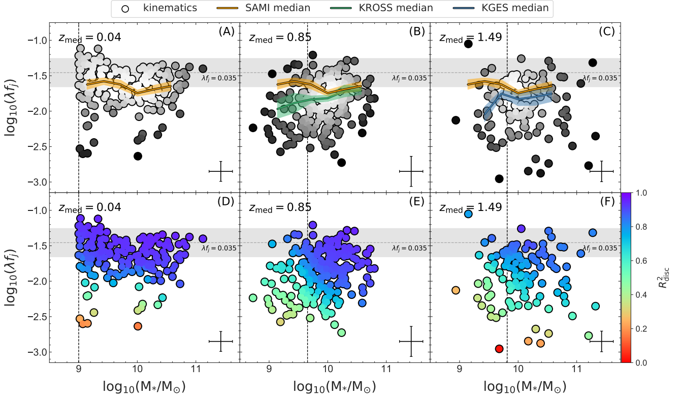
Figure 9. The product of the halo spin ( \lambda ) and the ratio of the total specific angular momentum of the disc to that of the halo ( f_j ) as a function of stellar mass for kinematics sub-sample galaxies at z \approx 0.04 , \approx 0.85 , and \approx 1.49 . In the top row the scatter points are colour-coded by the local spatial density of the points themselves (quantified via a Gaussian kernel density estimate and LOESS-smoothed). In the bottom row the scatter points are colour-coded by the corresponding galaxy’s “disciness”, R_{\text{disc}}^2 (with LOESS smoothing applied). The median trend for the SAMI galaxies, and its corresponding 1\sigma uncertainty, is displayed in each panel in the top row as the orange solid line and corresponding filled region, respectively. The median trends for the KROSS and KGES galaxies are displayed in respectively green and blue in the middle and right panel. The horizontal dashed grey line in each panel indicates the expected value if f_j = 1 and \lambda = 0.035 ( \pm 0.2 dex, indicated via the horizontal filled grey region), the latter according to (Macciò et al. 2008). In each panel we include a vertical dashed line representing the stellar mass above which each sample contain purely main sequence galaxies (see text for details). For main sequence star-forming galaxies, \lambda f_j does not significantly depend on stellar mass or redshift. It does however strongly depend on how “discy” a galaxy is (i.e. how disc-like its velocity field appears, as quantified by its R_{\text{disc}}^2 value).
