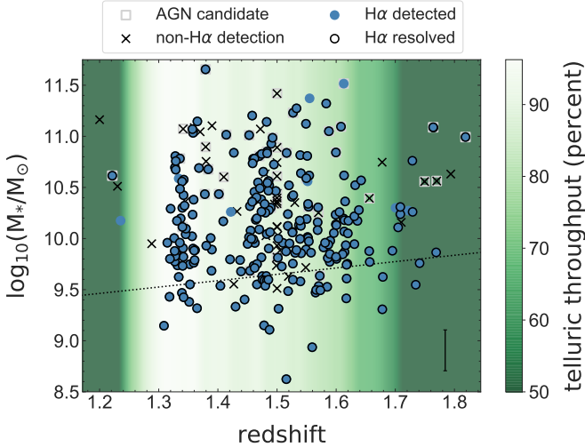
Figure 2. The stellar masses of the KGES galaxies as a function of their redshift (spectroscopic for H \alpha -detected systems, photometric otherwise). Symbols are as for Figure 1. The stellar mass error bar (assumed constant across the sample) is shown in the bottom right. The dotted black line represents the approximate stellar mass limit for star-forming galaxies corresponding to K = 23 at each redshift. The green shading in the background indicates the telluric throughput at the observed wavelength of H \alpha emission at the corresponding redshift (dark green to white: more severe to less severe telluric absorption). By design, the majority of H \alpha -detected galaxies are at redshifts corresponding to higher telluric throughput at the observed wavelength of H \alpha .
