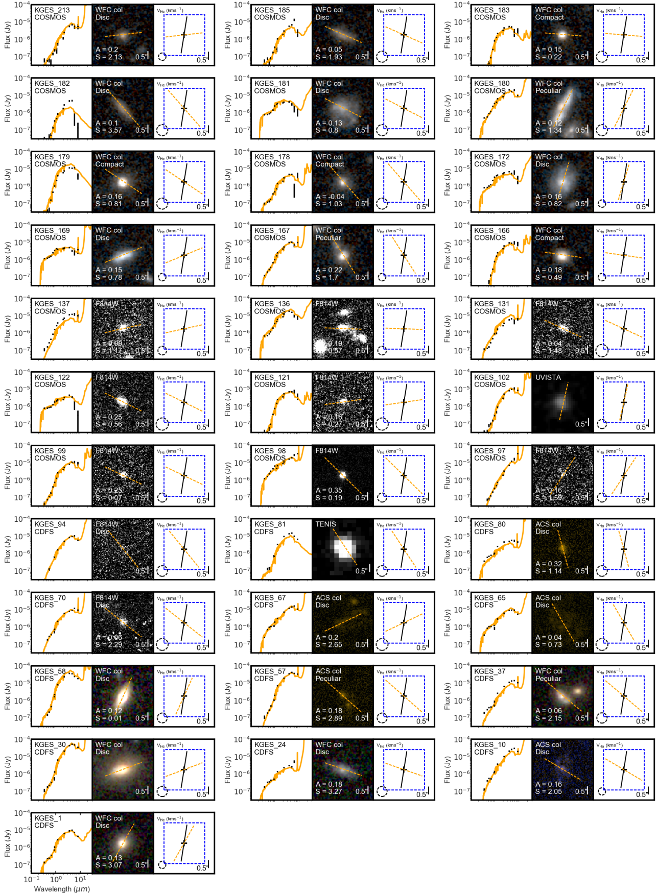
Figure A1. For each galaxy we show the multi-wavelength photometry from UV - 8\mu\text{m} with the derived MAGPHYS SEDs fits (left), the ‘best’ broadband image with semi-major axis (orange line) and asymmetry and clumpiness values stated (middle) and the H\alpha velocity map of the galaxy (right) with kinematic position angle (black line).
