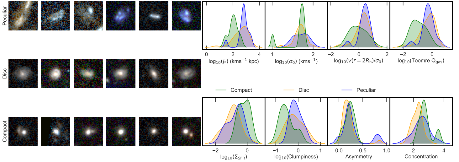
Figure 12. HST colour images of KGES galaxies in the stellar mass range 9.95 \leq \log_{10}(M_*/M_\odot) \leq 10.5 split into Compact, Disc and Peculiar morphological classes (left) with the kernel density distribution of specific angular momentum ( j_* ), velocity dispersion ( \sigma_0 ), ratio of rotation velocity to velocity dispersion ( V(2R_h)/\sigma_0 ), disc stability ( Q_{\text{gas}} ), \text{H}\alpha star formation rate surface density ( \Sigma_{\text{SFR}} ), Clumpiness, Asymmetry and Concentration (right). The velocity dispersion and concentration of Compact, Disc and Peculiar galaxies are very similar. Compact galaxies have lower specific stellar angular momentum, are more dispersion dominated, have lower Toomre Q_{\text{gas}} , are less clumpy, more asymmetrical but have higher \Sigma_{\text{SFR}} than Disc-like galaxies. Peculiar galaxies on average have the same specific stellar angular momentum, are similarly rotation dominated, but have lower Toomre Q_{\text{gas}} and are more clumpy, more asymmetrical but with higher \Sigma_{\text{SFR}} than Disc-like galaxies.
