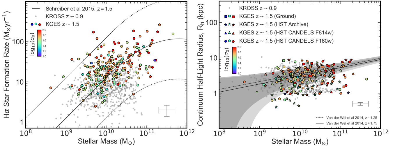
Figure 2. Left panel: The extinction corrected H\alpha star formation rate for the KGES sample as a function of stellar mass as derived from SED fitting using MAGPHYS (da Cunha et al. 2008). The KROSS z \sim 0.9 sample is shown as grey points in the background. The Schreiber et al. (2015) z = 1.5 star-formation rate stellar mass tracks, converted to a Chabrier IMF, are shown as well as factor 10 above and below the model track. Right: Stellar continuum half-light radii, derived from GALFIT, as a function of stellar mass. KROSS z \sim 0.9 sample shown as grey points in the background. Ground ( H , K ) imaging (squares), non-CANDELS HST imaging (stars), CANDELS HST F814W imaging (triangles) and, CANDELS HST F160W imaging (circles). The dashed and solid lines indicate the mass-size relation for star-forming galaxies at z = 1.25 and z = 1.75 respectively, as derived by van der Wel et al. (2014), with the shaded region indicating the uncertainty on the relations. The median uncertainty on stellar mass, star formation rate and stellar continuum size are shown by grey bars in the lower right corner of each panel and the distribution of velocity dispersion within the sample is shown by the colour bar. Both panels show that the star-formation rates and stellar continuum sizes of the KGES galaxies are ‘typical’ of star-forming galaxies at z \sim 1.5 .
